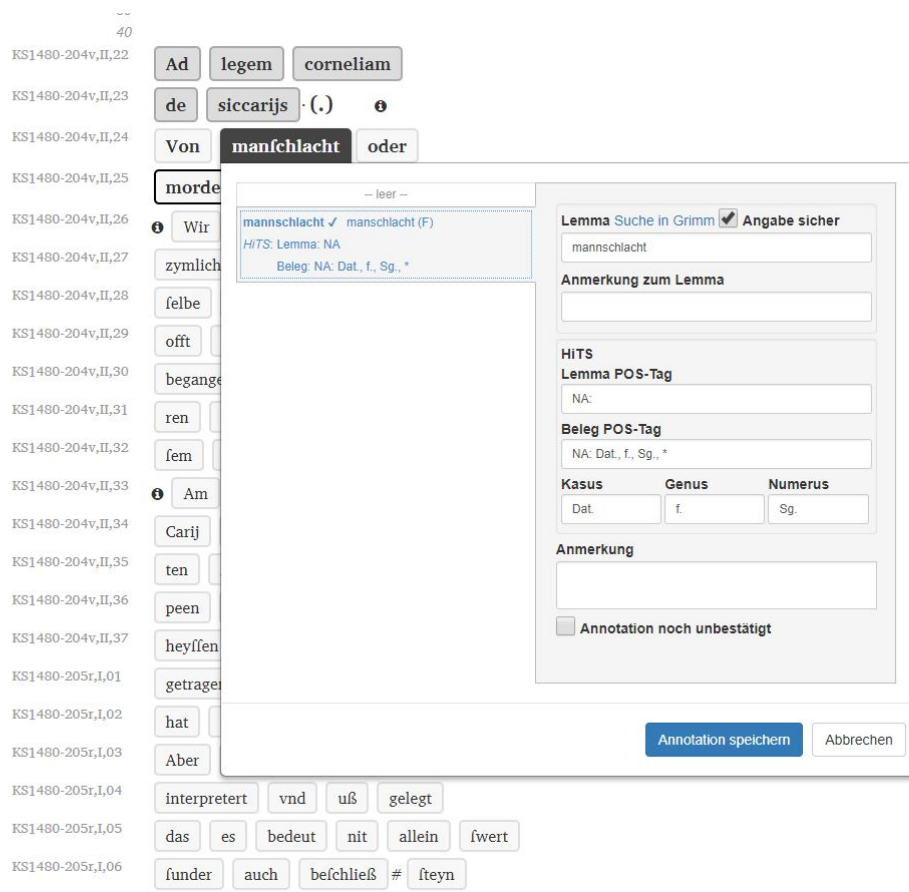
Annotation dialog in LAKomp.
